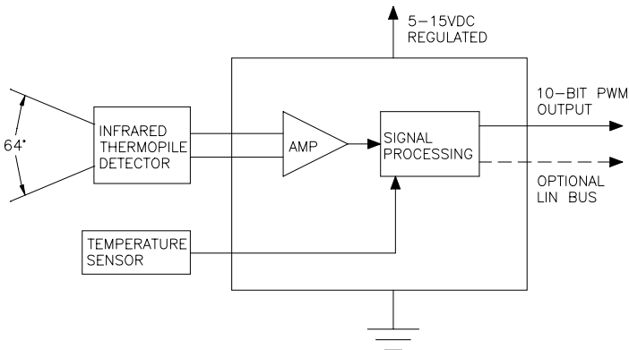
IR TEMPERATURE MODULE: BLOCK DIAGRAM
