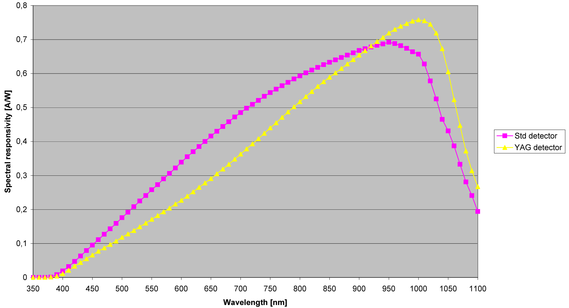
Spectral responsivity of various SiTek PSDs
